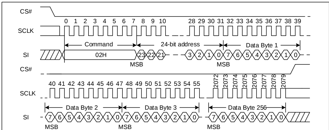
Figure 18. Page Program Sequence Diagram
