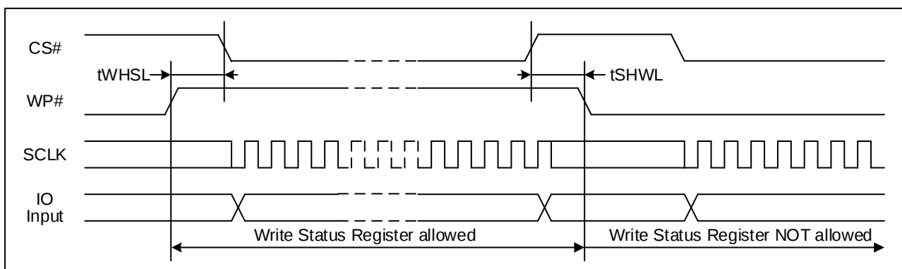
Figure 44. WP# Timing
