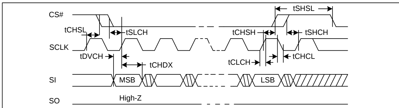
Figure 40. Input Timing
