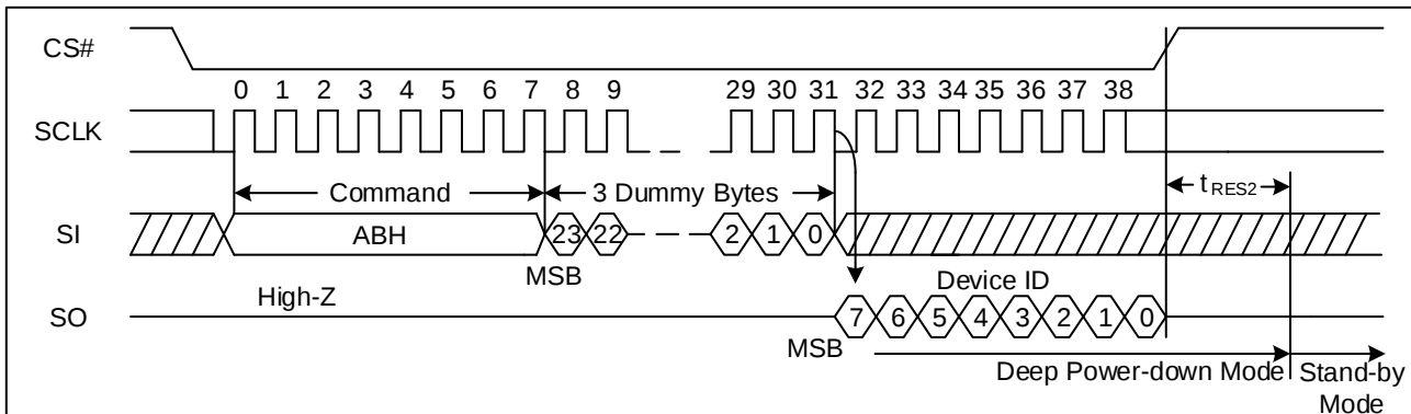
Figure 35. Release Power-Down/Read Device ID Sequence Diagram
