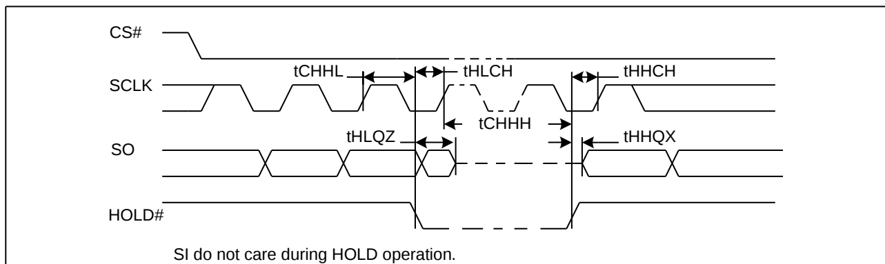
Figure 43. Hold Timing
