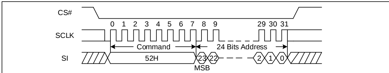
Figure 13. 32KB Block Erase Sequence Diagram
