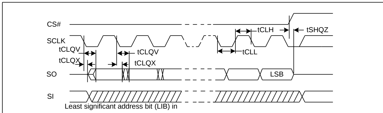
Figure 29. Output Timing
