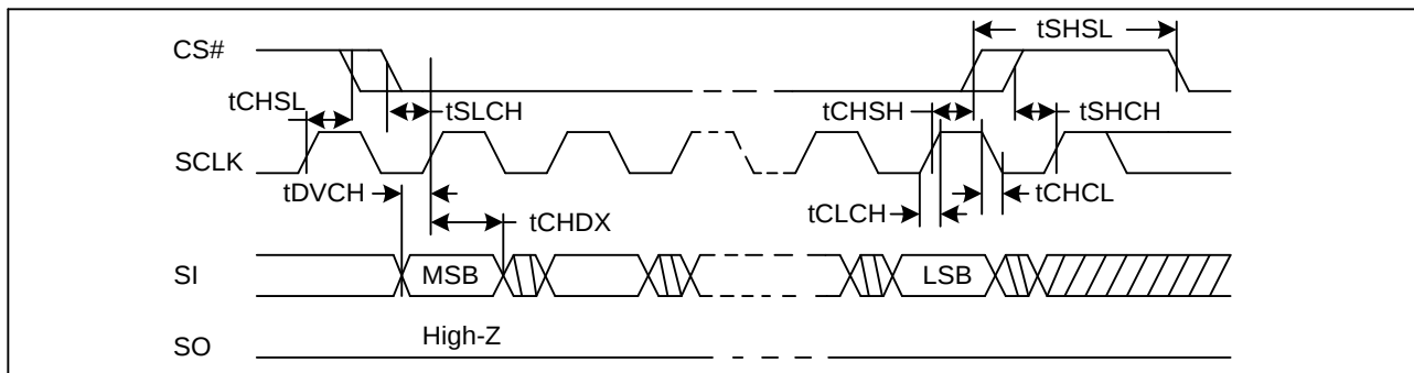
Figure 28. Input Timing
